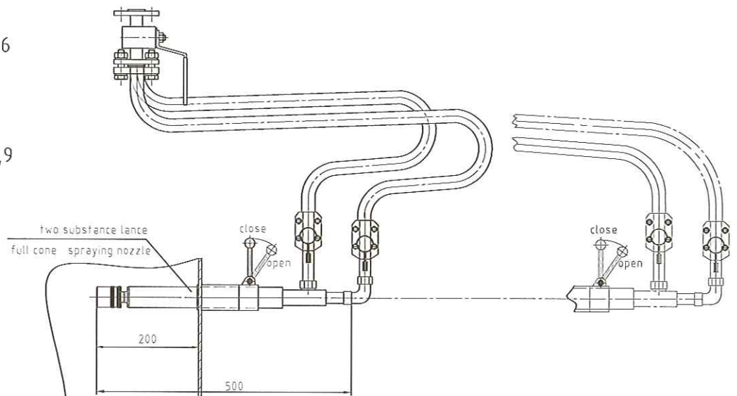
VIEW X
