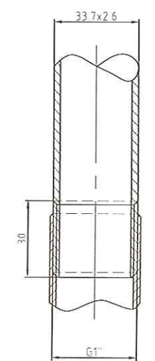
DETAIL Z M11
